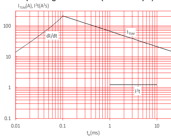
FIG.5: Non-repetitive surge peak on-state current for a sinusoidal pulse with width t_p < 20ms , and corresponding value of I^2t ( di/dt < 60A/\mu s )
